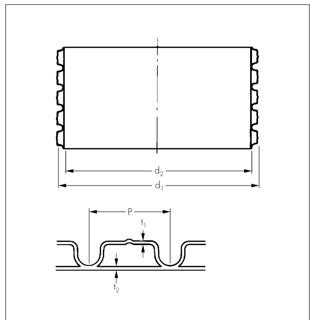
Figure 1 Twinwall pipe
