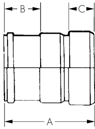
Adaptor twinwall or solid-wall PVC-U to clayware pipe
