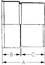
Adaptor (socket/spigot) twinwall pipe to solid-wall PVC-U socket (BS 4660/BS 5481)
