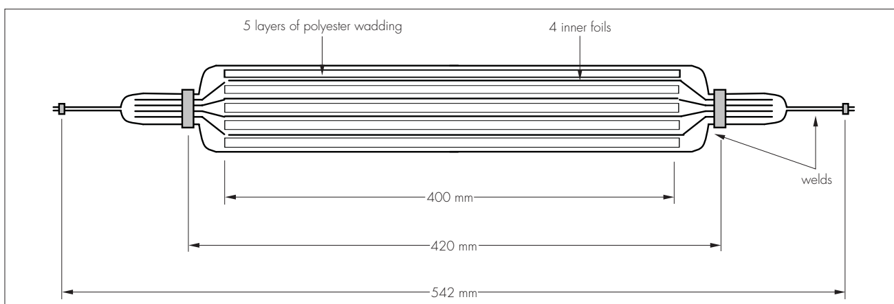
Figure 1 Rafterfit cross-section
