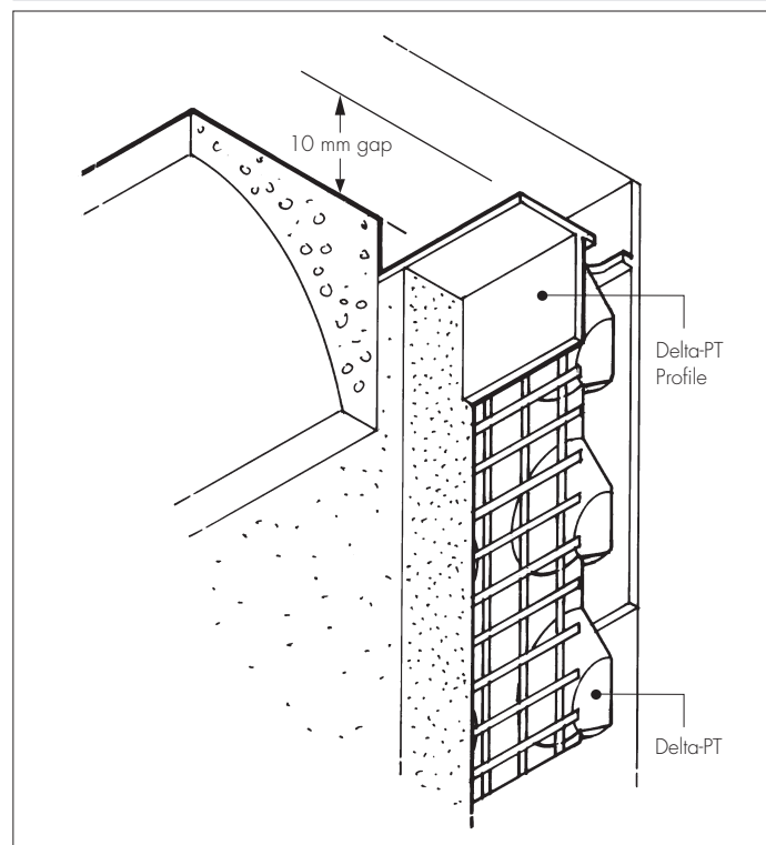
Figure 6 Coving details
