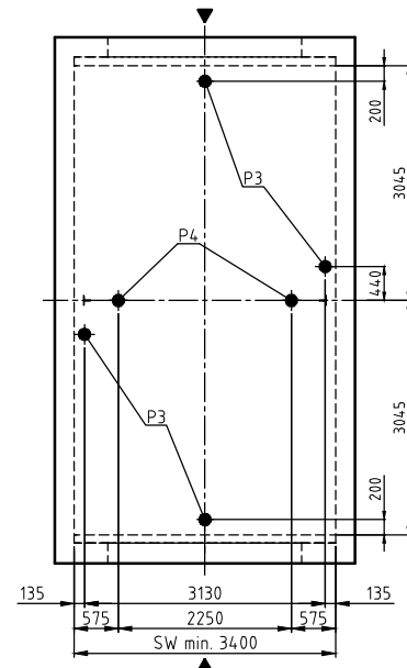
headroom with position liftingeyes M1:200
