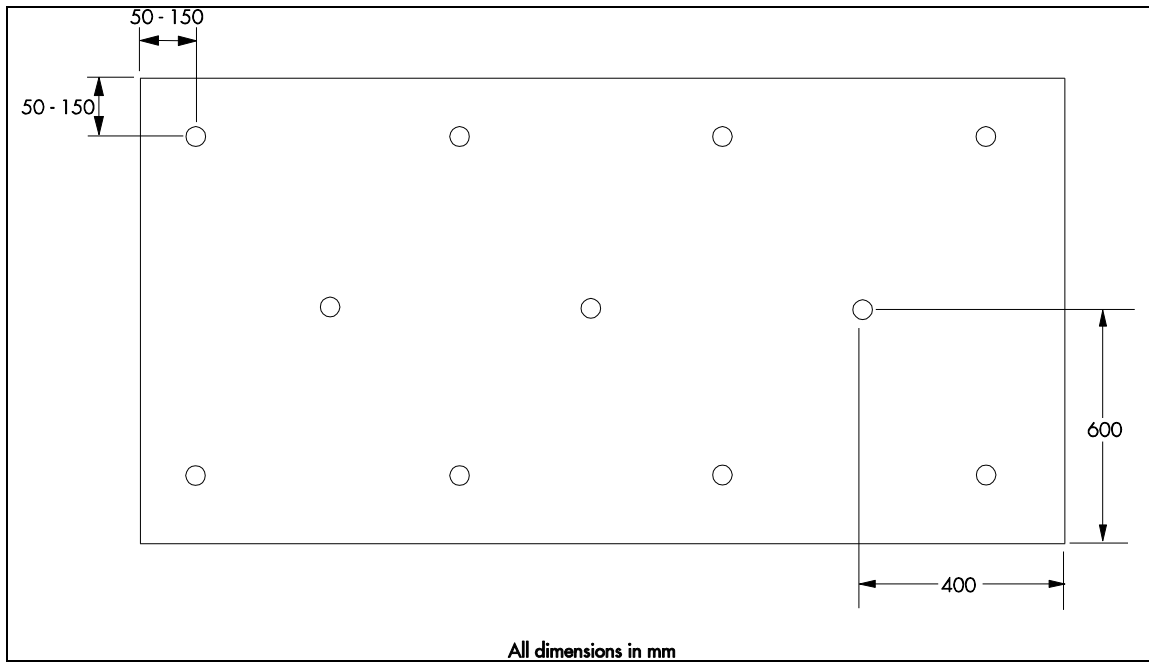
Figure 4 Fixing layout 2400 mm by 1200 mm board — minimum number of fixings
