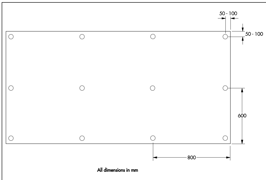
Figure 1 Fixing layout 2400 mm by 1200 mm board — minimum fixing numbers
