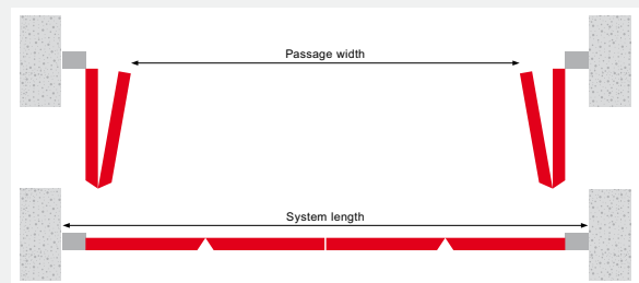
Plan view (installation between walls)
