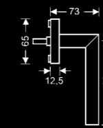
EF 284 Finish: satin stainless steel Matching lever: ER 28 Rhodos
