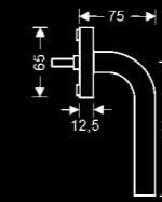
EF 254 Finish: satin stainless steel Matching lever: ER 25 Malta
