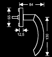
EF 264 Finish: satin stainless steel Matching lever: ER 26 Sylt
