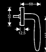
EF 244 Finish: satin stainless steel Matching lever: ER 24 Corfu
