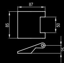
3 piece hinge EGB 402Q for glass doors Finish: polished stainless steel
