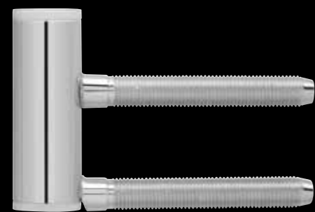
Frame inserts – EGB 3 V 4400 WF für wooden frame door Height: 48,5 mm Finish: zinc coated steel
