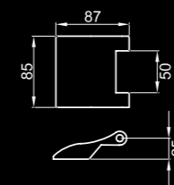
3 piece hinge EGB 302 for glass doors Finish: satin stainless steel
