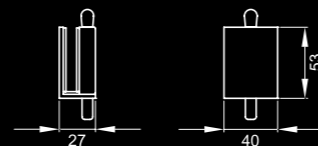
Slide over door bolt – EGF 100 with floor socket, for 8 -10 mm glass Finish: satin stainless steel
