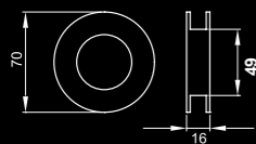
Sliding door handle for glass doors EZ1706 GS – EZ1706 GSH (for screwing) Drilling diameter: 50 mm Finish: satin stainless steel
