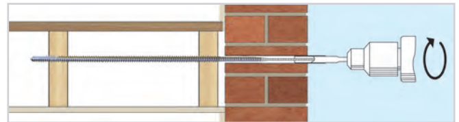
2. Fit the BowTie HD Support Tool to an SDS rotary hammer drill, insert the BowTie HD and drive it (off hammer) into, and through, the first and second joists
