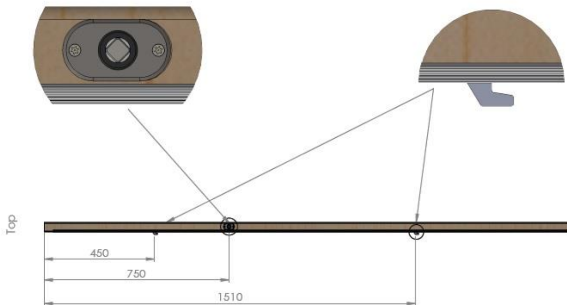
Stop Mounted Multilock, Lock and Hook Overview
