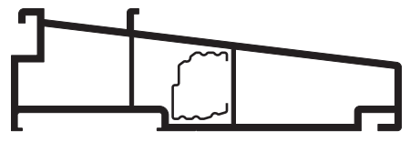
3S150 150mm Sill (G/Steel 3RS-V2)
