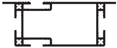
3CAV22 100mm Cavity Closer
