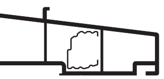
3S125 125mm Sill (G/Steel 3RS-V2)
