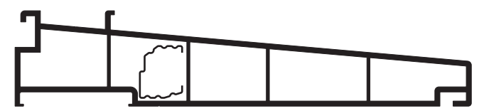
3S225 225mm Sill (G/Steel 3RS-V2)
