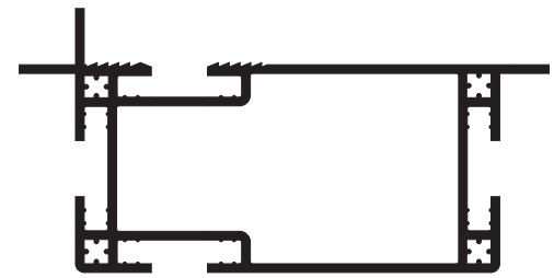
3CAV24 100mm Cavity Closer
