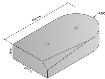
Transition Quadrant (LH shown)
