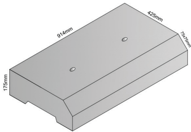
Cycle Segregation kerb
